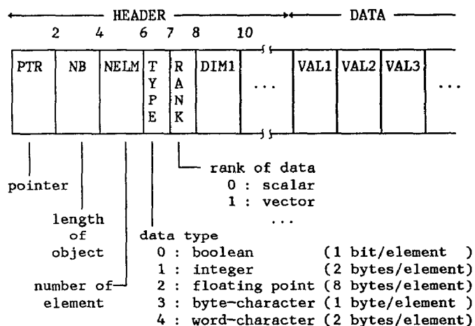
Figure 5. APL Data Format
